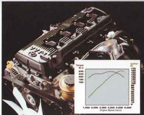
2TR-FE Max. Power: 160 Ps / 5,200 rpm Max. Torque: 241 Nm / 3,800 rpm
